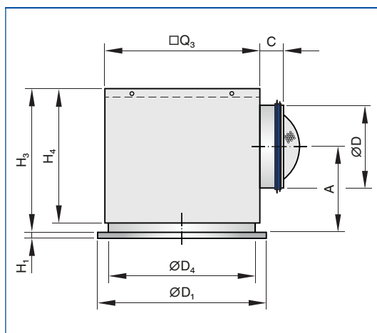
Circular diffuser face with plenum box for horizontal duct connection
