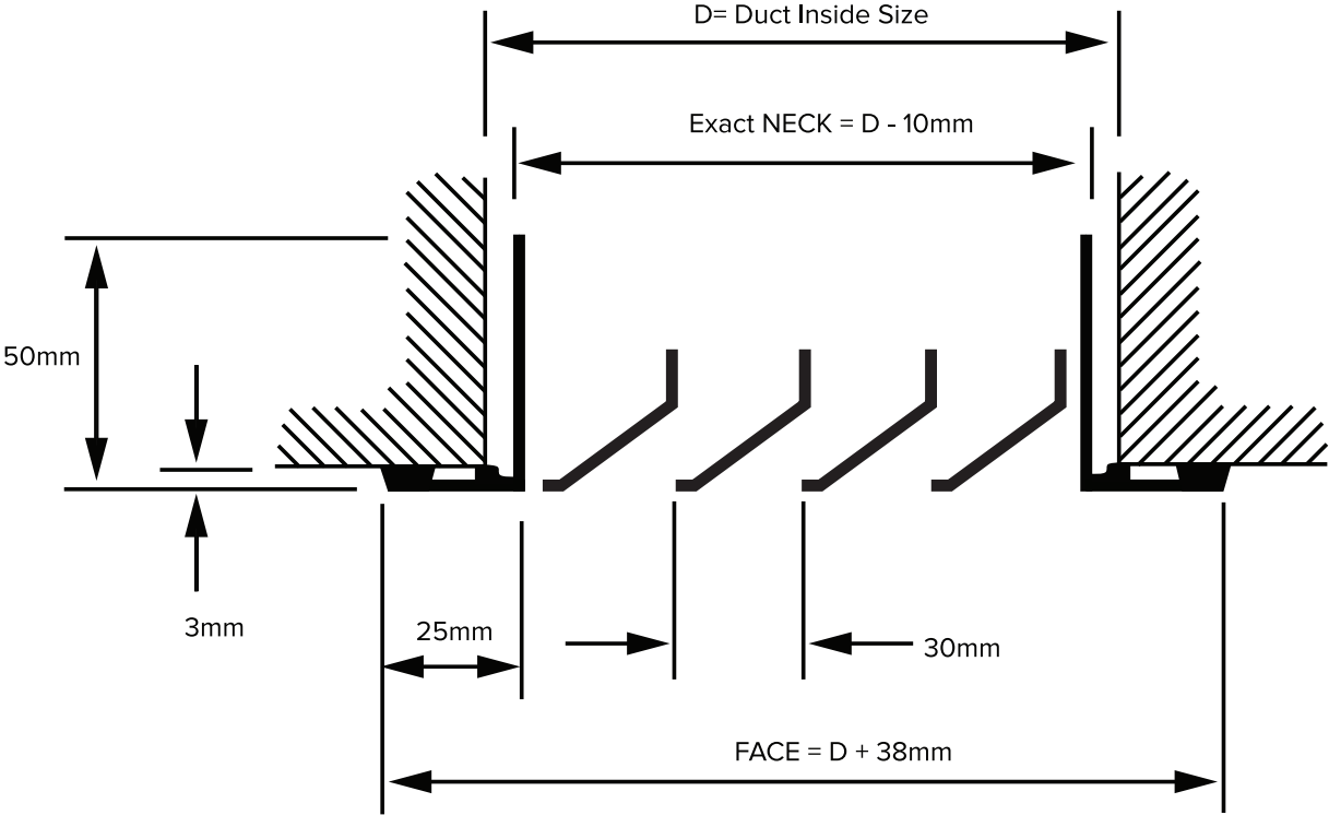
Cross sectional diagram
