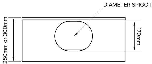
SIDE PROFILES - SWCB - 585-585
