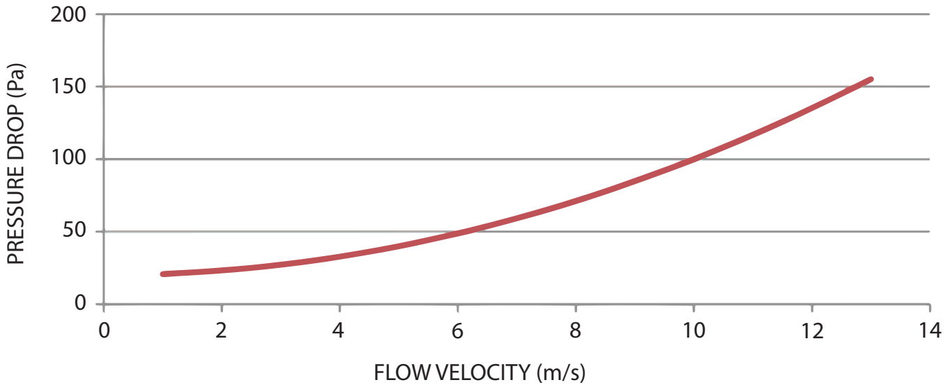
NON RETURN DAMPER (NRD) – PRESSURE DROP
