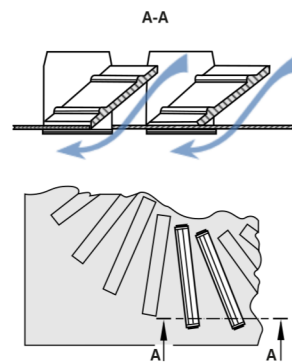
Air control blades set to internal swirl
