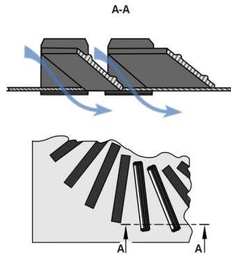
Air control blades set to external swirl
